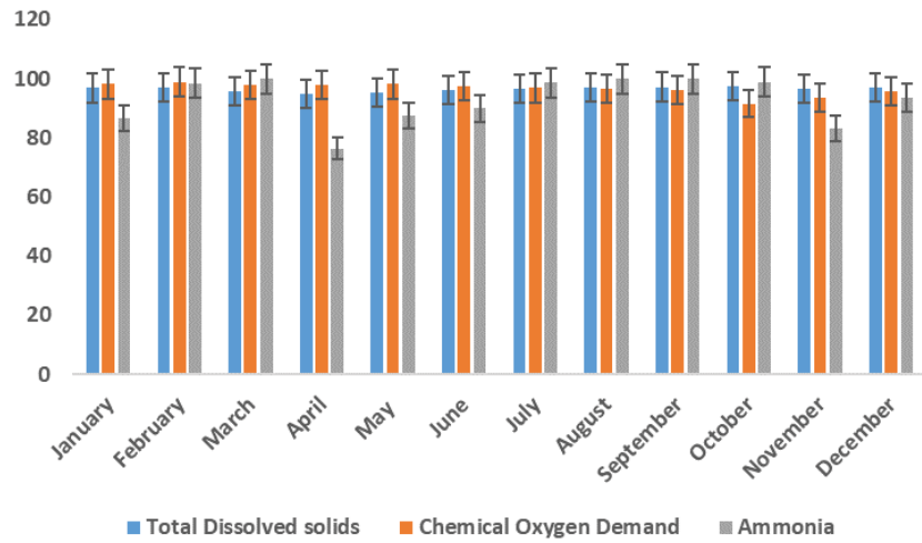
Fig. 6. Percentage reduction of TDS, COD and NH 3 -N RO 2018.
