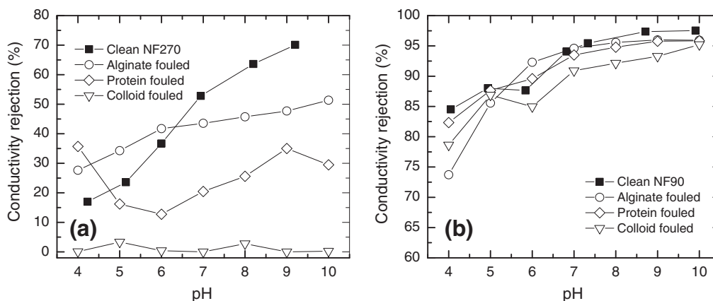
Fig. 4. Conductivity rejection by the (a) NF-270 and (b) NF-90 membranes under clean and fouled conditions as a function of pH.
