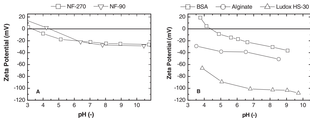
Fig. 1. (A) Zeta potential of the NF-270 and NF-90 membranes and (B) zeta potential of the model foulants (data from [6,23,30,31]).
