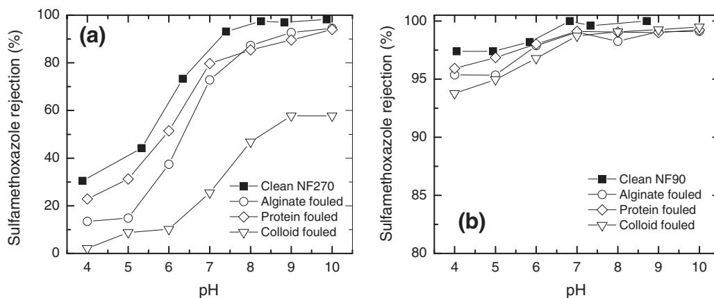
Fig. 5. Sulfamethoxazole rejection by the (a) NF-270 and (b) NF-90 membranes under clean and fouled conditions as a function of pH.
