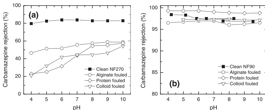
Fig. 6. Carbamazepine rejection by the (a) NF-270 and (b) NF-90 membranes under clean and fouled conditions as a function of pH.
