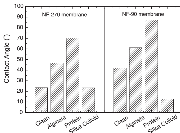
Fig. 3. Change in membrane surface hydrophobicity due to fouling of the NF-270 and NF-90 membranes. Experimental conditions are as in caption of Fig. 2.
