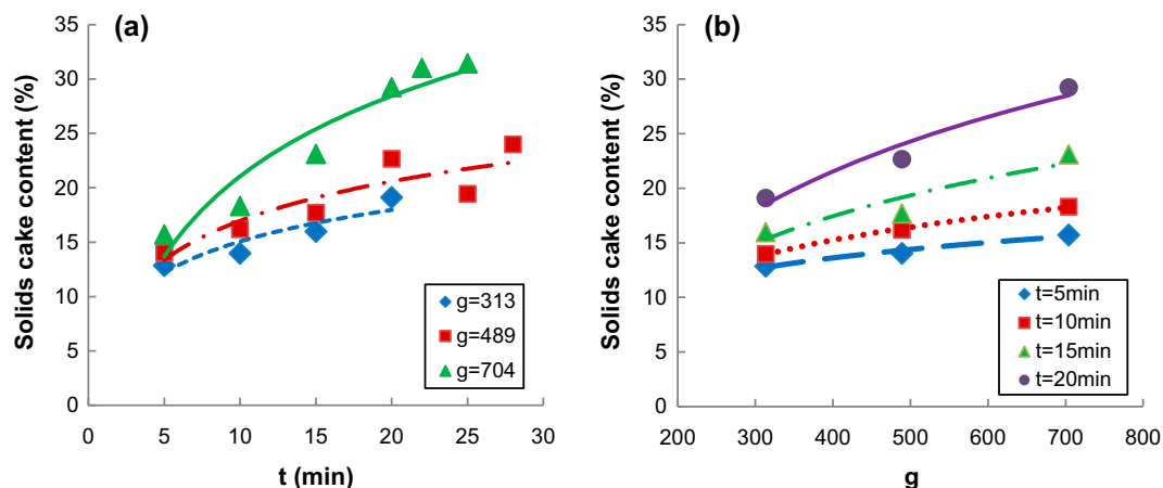
Fig. 4. Effects of (a) centrifugal speed and (b) centrifugal time on solids cake content.
