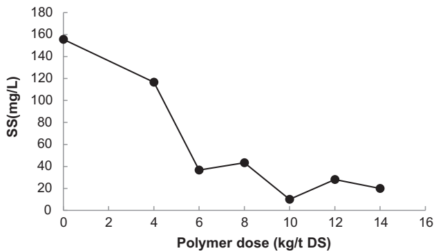
Fig. 7. Effect of polymer dose on SS in the filtrate from the modified centrifugal tests.
