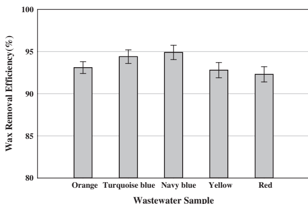
Fig. 2. Wax removal efficiency in single dye samples.
