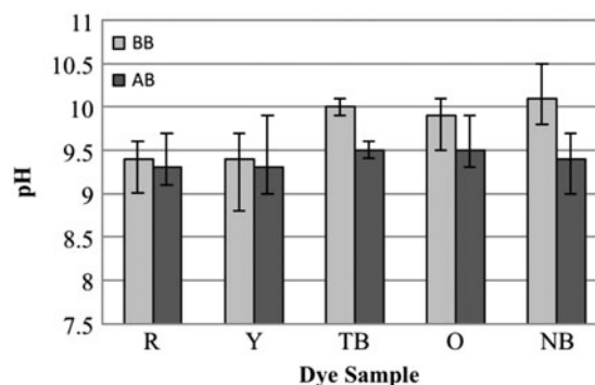
Fig. 8. pH removal efficiency in single dye wastewater samples.
