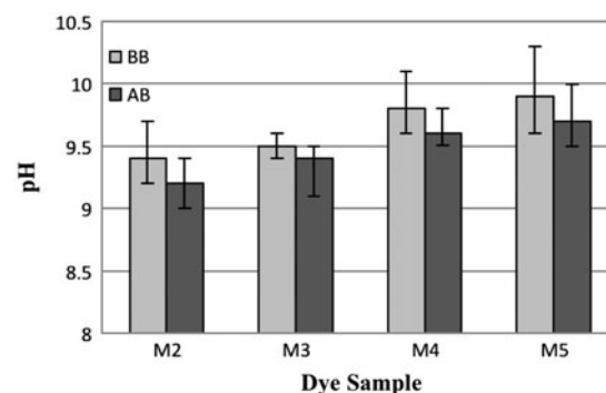
Fig. 9. pH removal efficiency in mixture dye wastewater samples.
