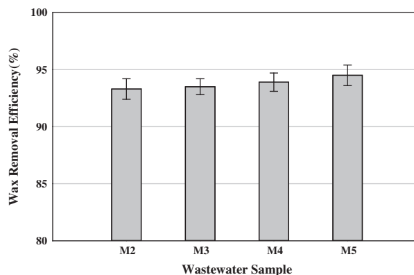
Fig. 3. Wax removal efficiency in mixture dyes samples.
