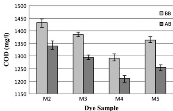
Fig. 5. COD removal efficiency in mixture dye wastewater samples.
