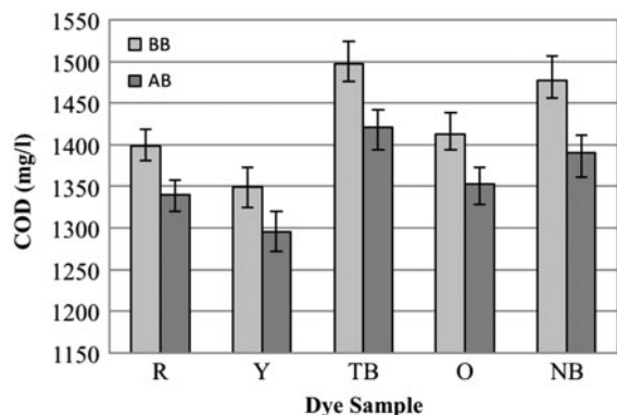
Fig. 4. COD removal efficiency in single dye wastewater samples.
