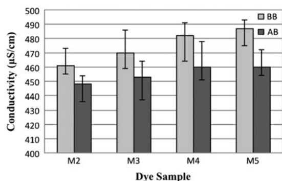
Fig. 7. Conductivity removal efficiency in mixture dye wastewater samples.
