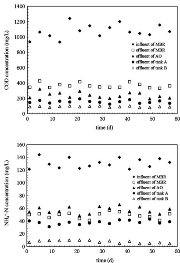
Fig. 4. Evolutions of COD and ammonia nitrogen concentrations during steady operation of the whole system.
