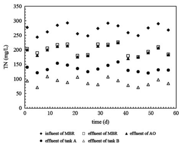
Fig. 5. Evolution of TN concentration during steady operation of the whole system.
