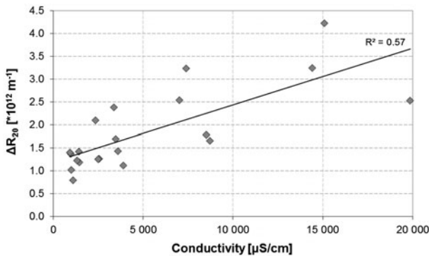
Fig. 6. Impact of salt concentration on activated sludge filterability.
