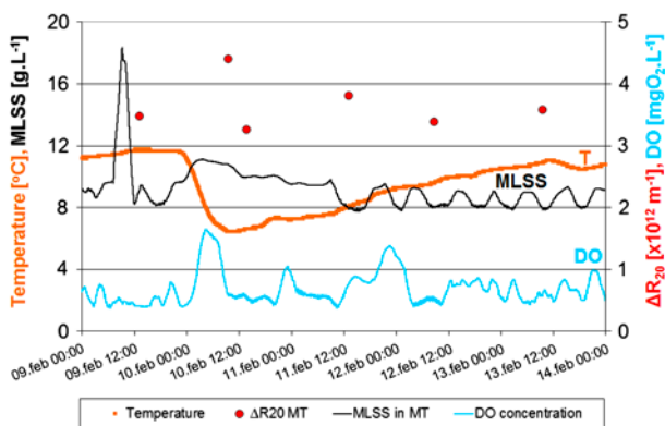
Fig. 3. Temperature, MLSS, DO profiles and \Delta R_{20} values measured at MBR Varsseveld during “winter 2009” campaign.
