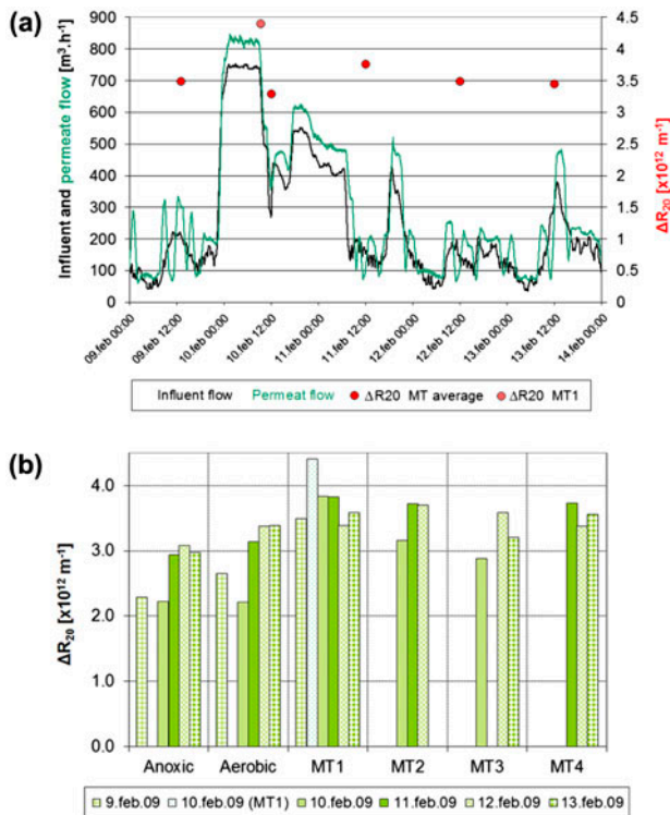
Fig. 1. (a) Influent and permeate flows as well as average daily \Delta R_{20} values for membrane tank samples vs. operational time and (b) corresponding activated sludge filterability development in the various compartments of the MBR Varsseveld during different days of the “winter 2009” campaign. On Fig. 1(a), a single measurement of the sludge sample from the membrane tank #1 (MT1), the only one corresponding to the actual peak flow is plotted.
