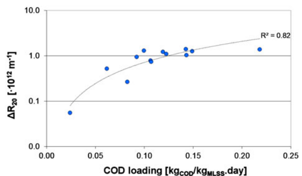
Fig. 9. Filterability of activated sludge vs. influent specific COD loading in Heenvliet municipal MBR.
