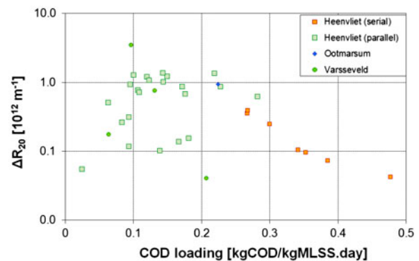
Fig. 8. Filterability vs. specific COD loading in municipal MBRs. Term “serial” refers to serial MBR configuration and indicates operation of the MBR in series to the CAS system.
