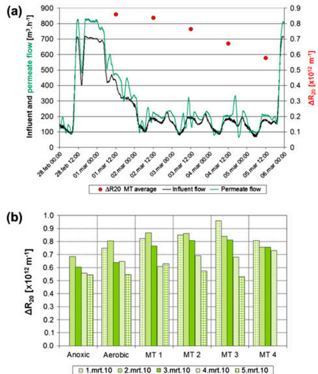
Fig. 2. (a) Influent and permeate flows as well as average daily \Delta R_{20} values for membrane tank samples vs. operational time and (b) corresponding activated sludge filterability development in the various compartments of the MBR Varsseveld during different days of the “winter 2010” campaign.
