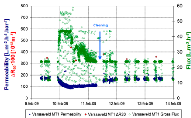
Fig. 4. Varsseveld MBR operation monitoring—Flux, permeability and filterability—During winter 2009. The graphs illustrate process permeability plotted on y -axis (in blue), sludge filterability expressed as, and for better visualization multiplied by a factor 100, \Delta R_{20} parameter on y -axis (in red), gross flux on second y -axis (in green) and time on x -axis.
