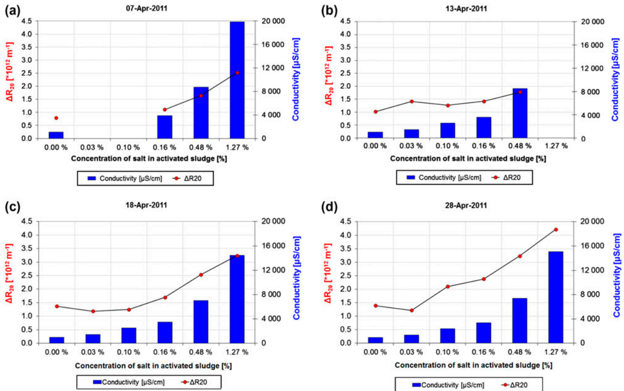
Fig. 5. Activated sludge filterability vs. conductivity.
