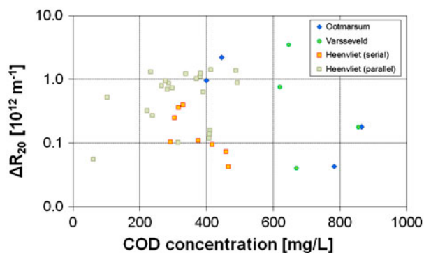
Fig. 7. Filterability vs. influent COD concentration in municipal MBRs.
