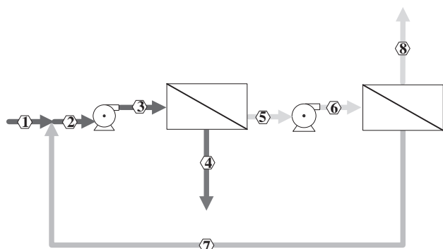
Fig. 1. Full second pass flow diagram.
