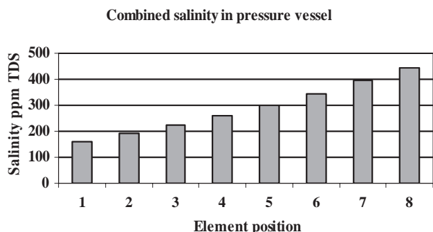
Fig. 3. Combined salinity in 8 elements seawater reverse osmosis (SWRO) pressure vessel.
