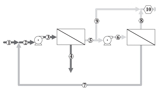
Fig. 2. Partial second pass flow diagram.
