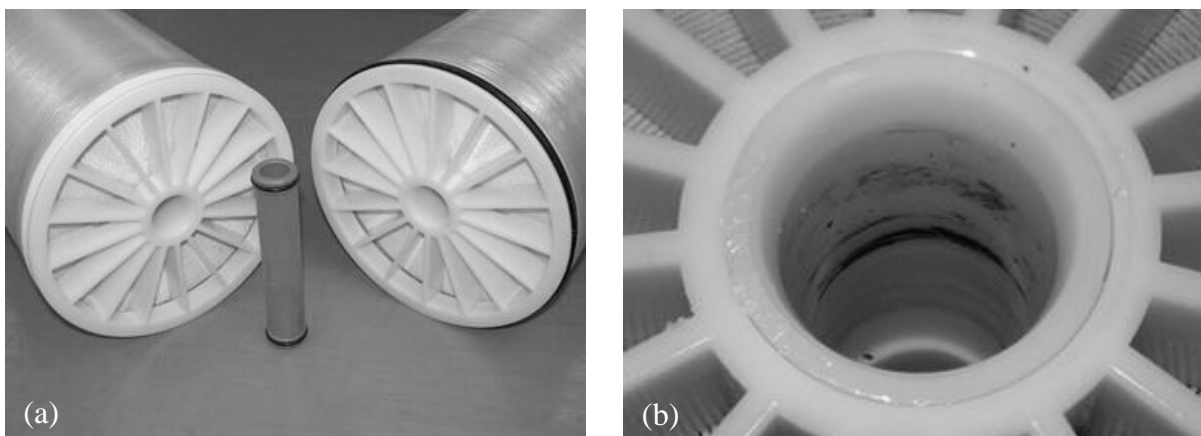
Fig. 9. (a) Standard sliding coupler used to connect the permeate tubes of adjacent elements; (b) Residue from o-ring abrasion.
