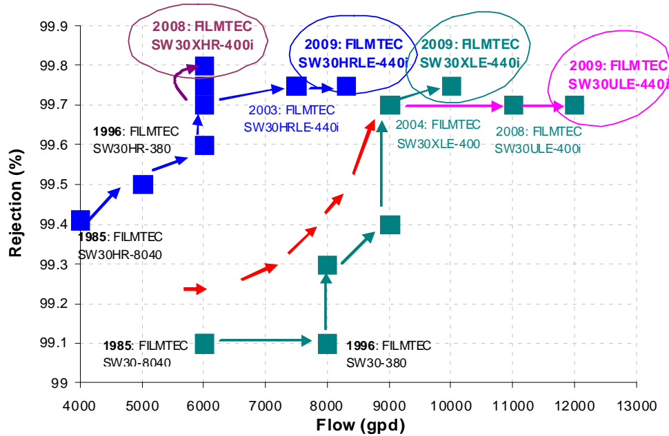
Fig. 2. Evolution of spiral wound module performance, illustrated by example of the DOW™ FILMTEC™ seawater desalination product range.
