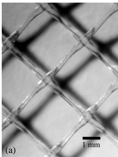
Fig. 4. (a) Biplanar extruded netting is comprised of two intersecting sets of parallel, extruded strands; (b) An early patent was obtained by Nalle [19].
