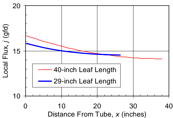
Fig. 8. Variation in local membrane flux with leaf coordinate (distance from permeate collection tube) P = 0.05 gfd/psi, k = 130 psi-s/in 3 , j_{avg} = 15 gfd.
