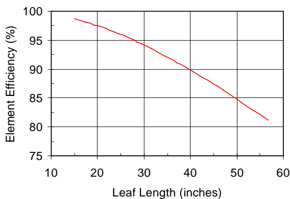
Fig. 7. Effect of leaf length upon element efficiency P = 0.05 gfd/psi, k = 130 psi-s/in 3 .
