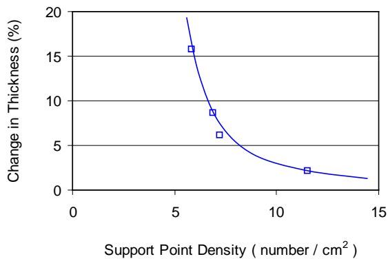
Fig. 5. Effect of support point density upon change in apparent thickness of feed spacer during module fabrication.
