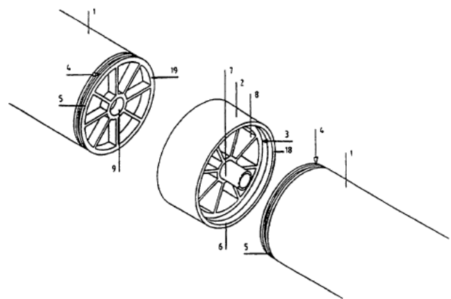
Fig. 11. Method of interconnection which eliminates the pressure vessel.
