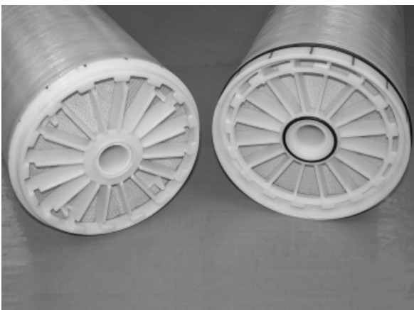
Fig. 10. Interlocking endcaps.
