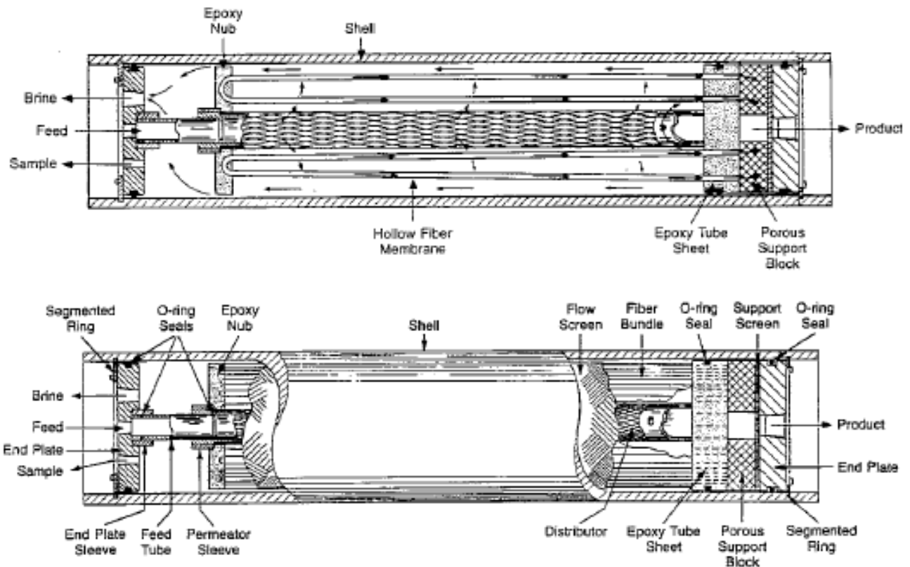
Fig. 1. Hollow fine fiber module and process [1].
