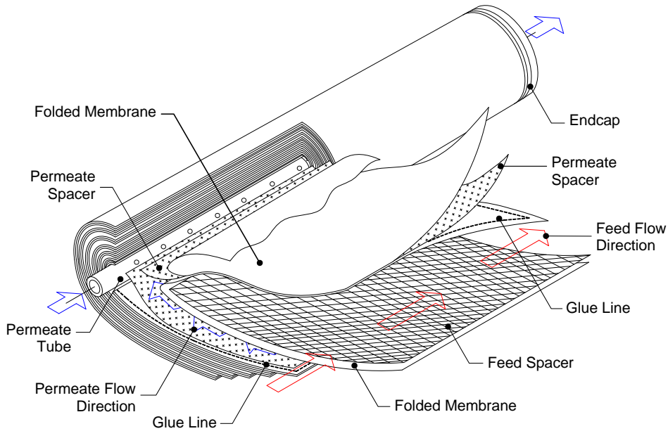
Fig. 3. Configuration of spiral wound membrane module for reverse osmosis.
