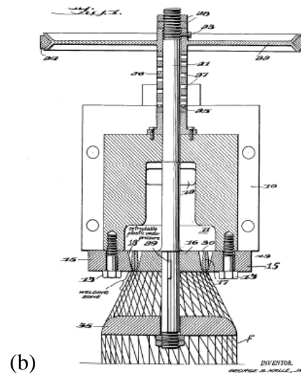
Fig. 4. (a) Biplanar extruded netting is comprised of two intersecting sets of parallel, extruded strands; (b) An early patent was obtained by Nalle [19].
