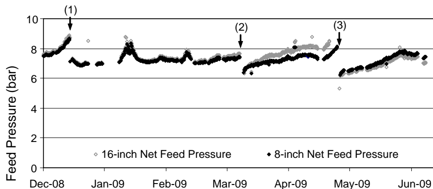
Fig. 13. Comparison of net feed pressure for 8-inch and 16-inch systems operated at 20.5 l/mh. Chemical cleaning of both trains was performed at (1,2,3).
