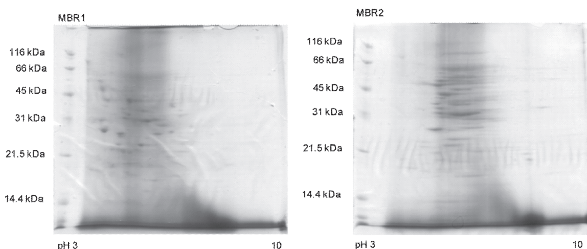
Fig. 3. 2D-PAGE images of foulants extracted from fouled membranes. Protein sample loading: MBR1, 310 \mu\text{g} ; MBR2, 240 \mu\text{g} .
