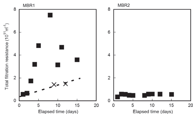
Fig. 1. Changes in total filtration resistance during the continuous operation. Crosses represent filtration resistances recorded just after physical membrane cleaning.
