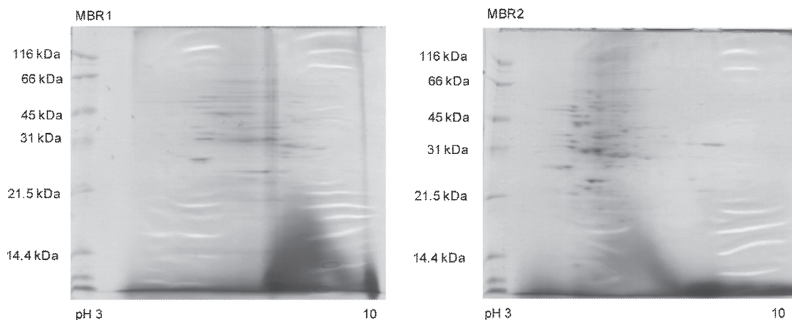
Fig. 2. 2D-PAGE images of dissolved organic matter contained in mixed liquor suspension of pilot-scale MBRs. Protein sample loading: MBR1, 200 \mu\text{g} ; MBR2, 210 \mu\text{g} .
