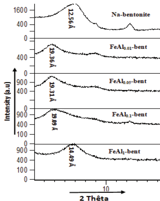
Fig. 1. X-ray diffraction spectra of raw and pillared bentonites.
