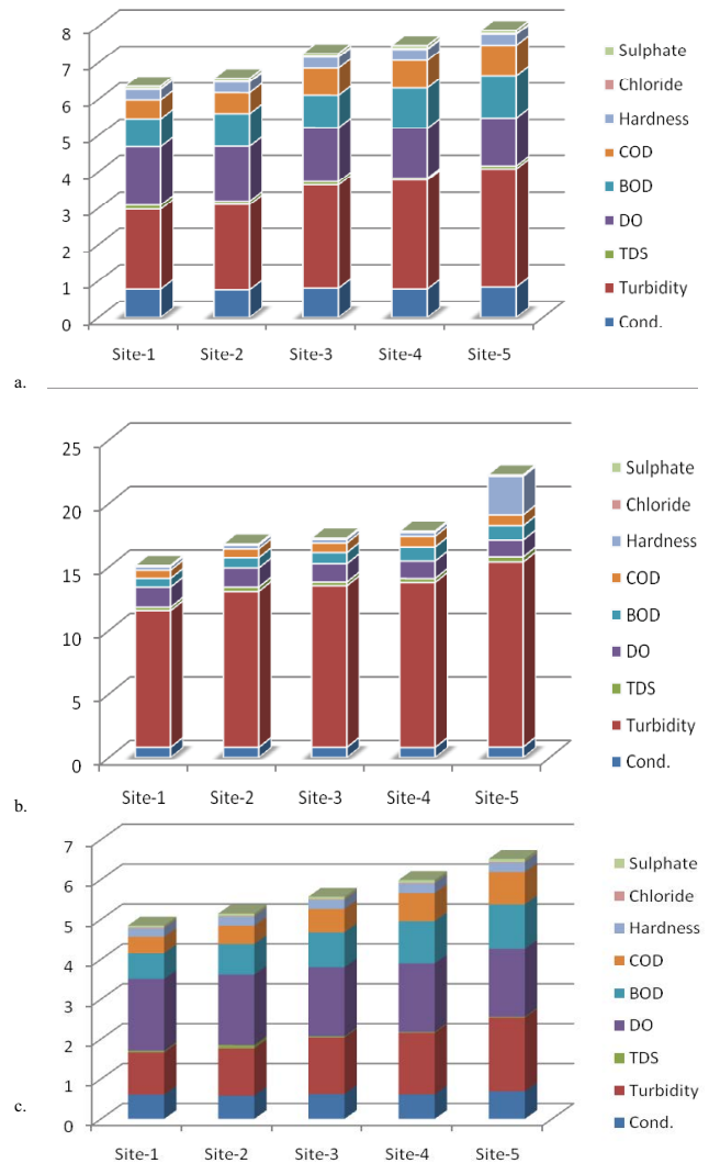
Fig. 2. PI of water quality parameters during summer (a), monsoon (b) and winters (c).
