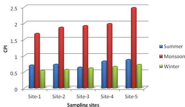
Fig. 3. Variation of CPI during summer, monsoon and winter.
