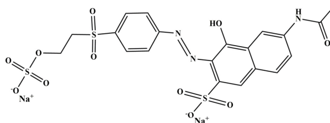
Fig. 1. Molecular structure of RO16.
