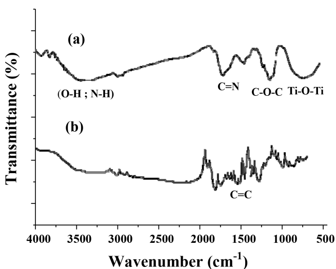
Fig. 14. FTIR spectra for (a) Chi-Gly/TNC-50 before adsorption and (b) Chi-Gly/TNC-50 after adsorption of RO16 dye.
