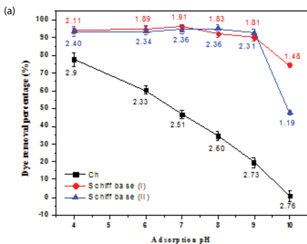
Fig. 10. (a) Effect of the adsorption’ pH on the removing percent (%) of MO using chitosan (Ch), chitosan Schiff base (I) and chitosan Schiff base (II) adsorbents (5 ppm MO, 180 min, 25°C, 250 rpm, 0.05 g) and (b) theoretical MO removal percent of the chitosan Schiff base (I) and chitosan Schiff base (II) adsorbents.
